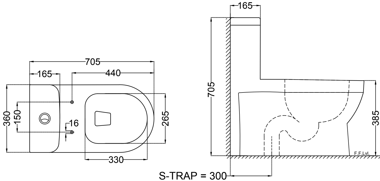
TOP VIEW
