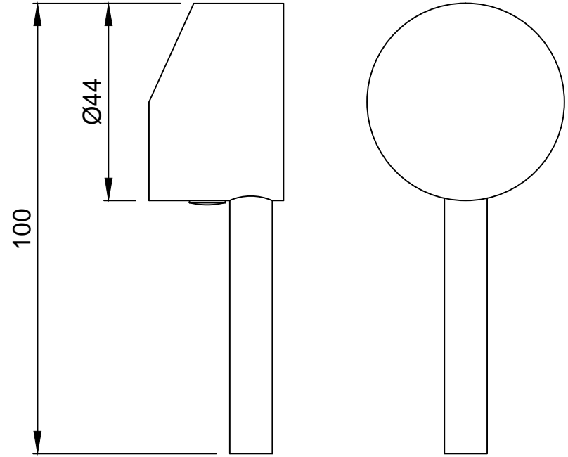
OPERATING LEVER
